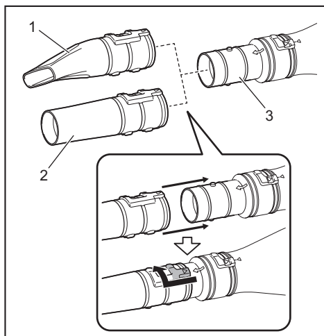
► 1. Flat nozzle 2. Extension nozzle 3. Adapter pipe
